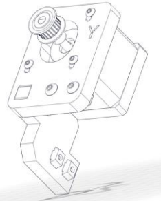
Y-motor
